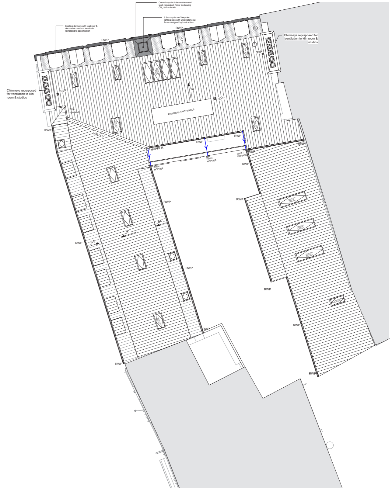
Roof Plan
